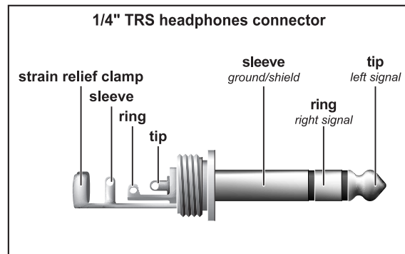
Fig. 4.6: 1/4" TRS connector for headphones
