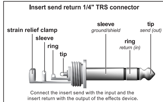
Fig. 4.5: Insert send return 1/4" TRS connector
