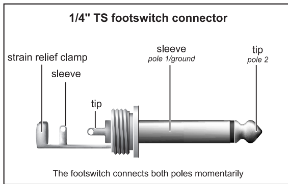
Fig. 4.1: 1/4" TS footswitch connector
