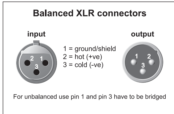
Fig. 4.2: XLR connections
