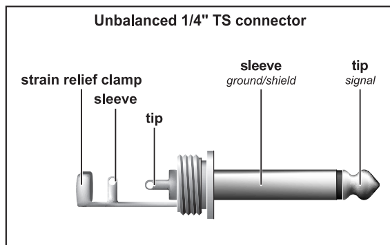
Fig. 4.3: 1/4" TS connector
