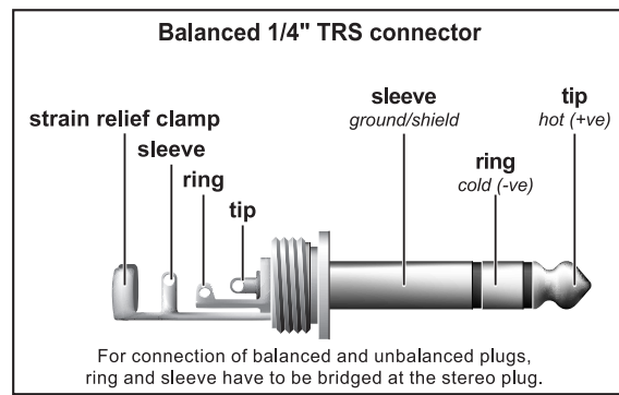
Fig. 4.4: 1/4" TRS connector
